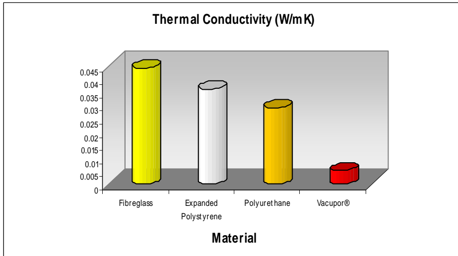
Indication of Vacupor's Superior Insulating Properties
